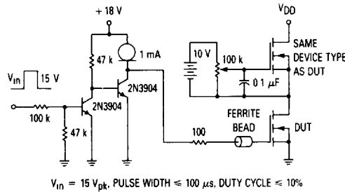
Figure 17. Gate Charge Test Circuit
